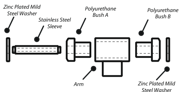
Figure 2 - Assembly
